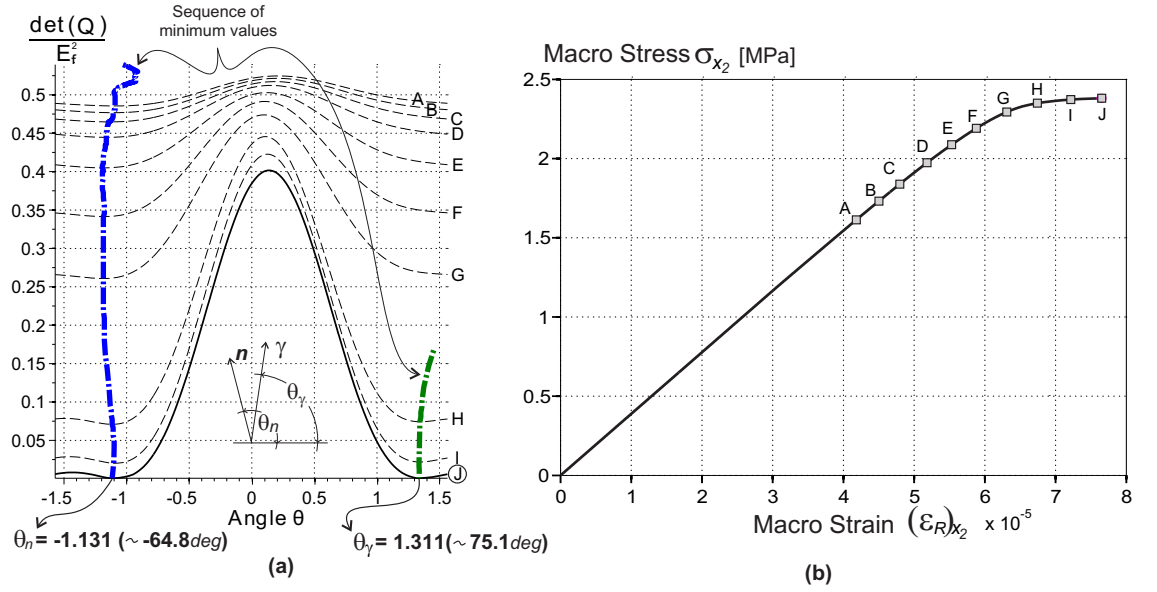
Figure 10: Analysis of the strain localization mode. a) Evolution of \det \mathbf{Q}(\mathbf{n}(\theta), t) for the \text{Cell}_{1 \times 1} with periodic boundary conditions. b) homogenized macro stress vs. macro strain. Letters identify the time when \det \mathbf{Q} has been evaluated.
