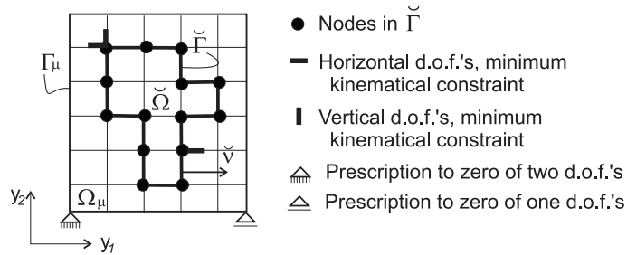
Figure 6: Micro-cell \Omega_\mu and finite element mesh with a null average value of the strain fluctuation increments in the region \check{\Omega} bounded by the curve \check{\Gamma} .
