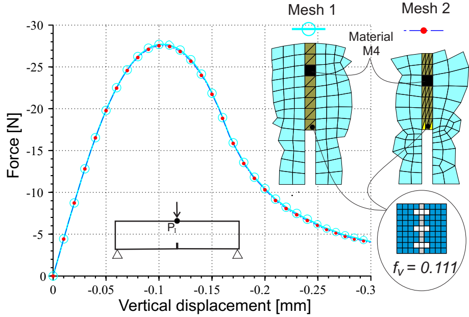
Figure 20: Load vs. vertical displacement of the load application point P_I . MS Models with two macroscopic mesh sizes.
