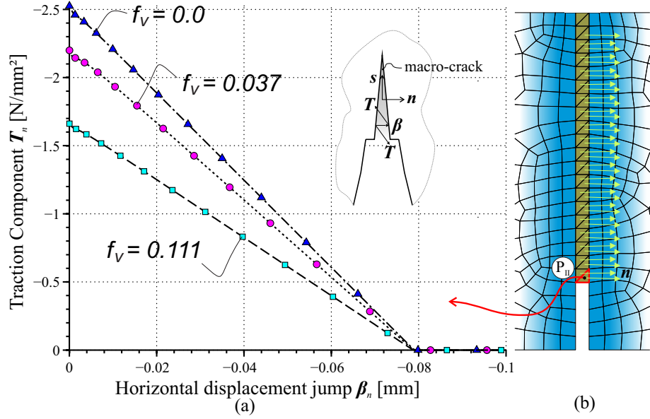
Figure 19: MS model. Horizontal-components of the traction vectors vs. horizontal displacement jump evaluated in the first point (picture-b) satisfying the bifurcation condition.
