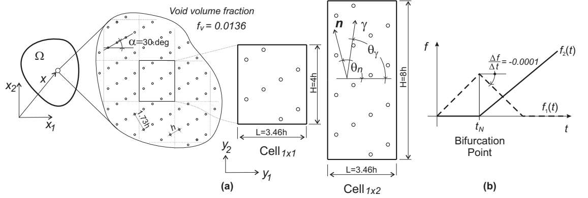
Figure 9: Fracture process analysis of a heterogeneous material point. a) Material microstructure and Cell definitions, b) pseudo-time dependent curves defining the evolution of the macrostrains.
