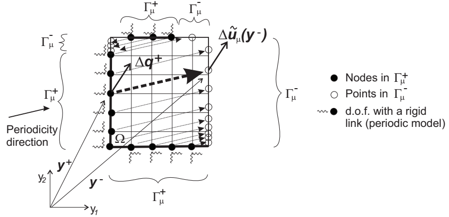
Figure 7: Micro-cell \Omega_\mu and finite element mesh. Hybrid boundary condition: periodicity along arbitrary directions which satisfies a null strain fluctuation increments in the region bounded by the curve \Gamma_\mu .
