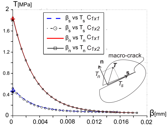
Figure 15: Normal and tangential components of the homogenized traction vector \mathbf{T} as a function of the macroscopic displacement jump \beta : Cell 1x1 and Cell 1x2 : periodic sub-model during the stable macroscopic regime.
