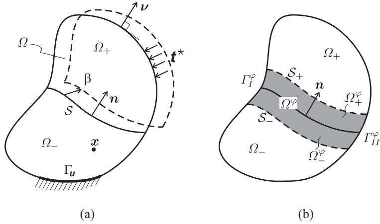
Figure 3: Mechanical problem exhibiting a strong discontinuities across the material surface \mathcal{S} .
