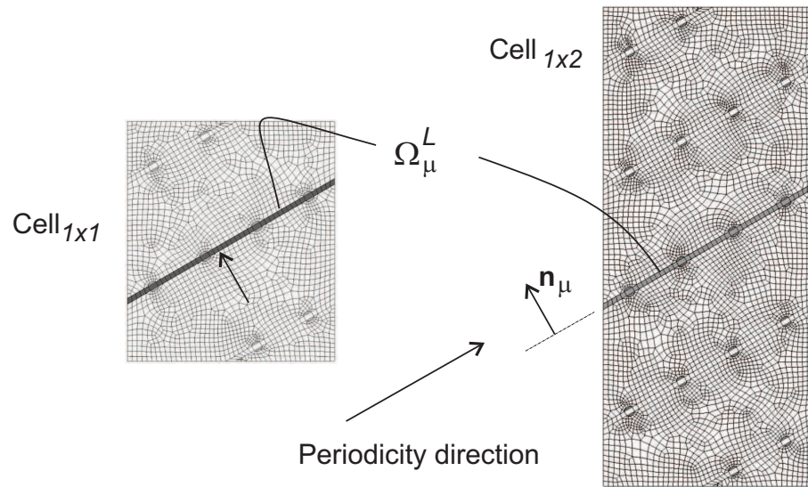
Figure 13: Finite element meshes for the cells: \text{Cell}_{1x1} and \text{Cell}_{1x2} . The strain localization domain \Omega_{\mu}^L is depicted in both cases.
