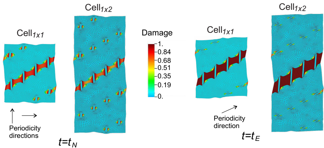
Figure 14: Micro-cell problem with fracture. \text{Cell}_{1x1} and \text{Cell}_{1x2} deformed meshes and damage distribution in two stages of analysis.
